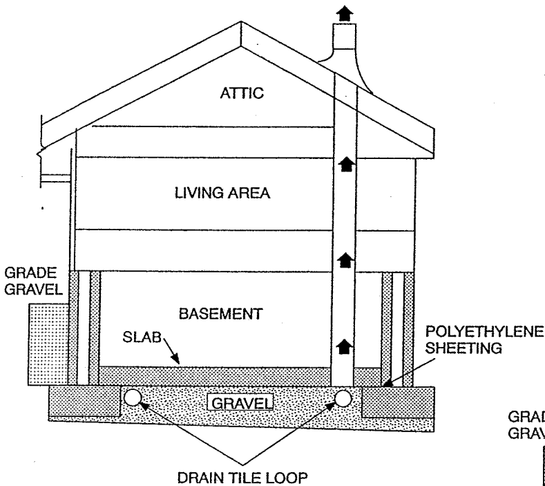
FIGURE AF102 RADON-RESISTANT CONSTRUCTION DETAILS FOR FOUR FOUNDATION TYPES
