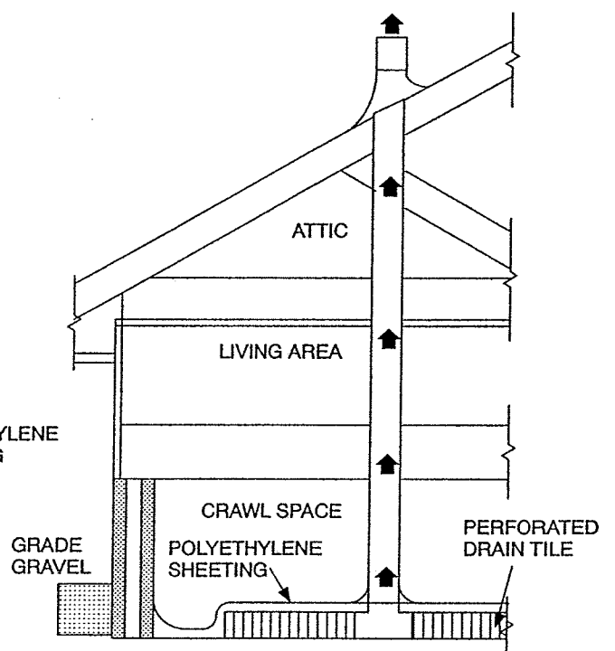
FIGURE AF102 RADON-RESISTANT CONSTRUCTION DETAILS FOR FOUR FOUNDATION TYPES
