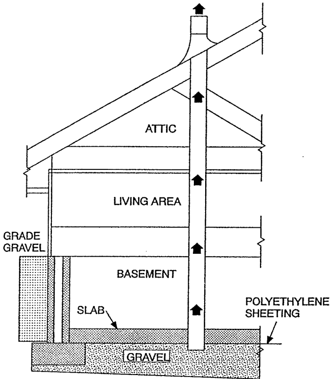
TYPICAL SUB-SLAB DEPRESSURIZATION PASSIVE RADON SYSTEM
